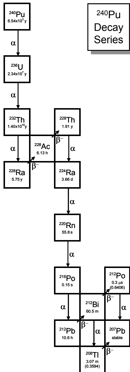
Figure 11.2 Decay series for 240 Pu. The half-life is shown directly below the isotope that is subject to decay; y = years, h = hours, d = days, m = minutes, s = seconds, μs = microseconds, stable = non-radioactive isotope. Decay half-life data were obtained using the WinChain program that provides electronic access to the ICRP38 Nuclear Decay Data Files (ICRP, 1983; Eckerman et al., 1994). WinChain is a public domain software application available for download from Oak Ridge National Laboratory ( http://ordose.ornl.gov/downloads.html ).
