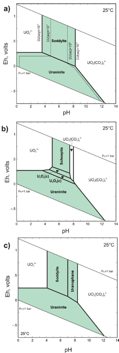
Figure 6.5 Eh-pH diagrams for U at 25°C. (a) System U-O-H-Si-C, with a\text{H}_4\text{SiO}_4 = 10^{-4.0} and \text{PCO}_2 = 10^{-2.5} bar. (b) System U-O-H-C with \Sigma\text{U} = 10^{-5} and \text{PCO}_2 = 10^{-2.5} bar. (c) System U-O-H-C-Na-Ca with \Sigma\text{U} = 10^{-5} , a\text{H}_4\text{SiO}_4 = 10^{-4.0} , and \text{PCO}_2 = 10^{-2.5} bar. Soddyite = (\text{UO}_2)_2\text{SiO}_4 \cdot 2\text{H}_2\text{O} ; uraninite = \text{UO}_2 ; schoepite = \beta\text{-UO}_3 \cdot 2\text{H}_2\text{O} ; uranophane = \text{Ca}(\text{H}_3\text{O})_2(\text{UO}_2)_2(\text{SiO}_4)_2 \cdot 3\text{H}_2\text{O} .
